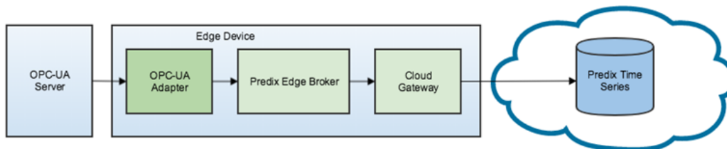
Figure 3. OPC-UA Sample Use Case
