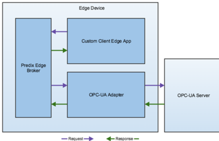
Figure 4. OPC-UA Command Handler Operation Steps
