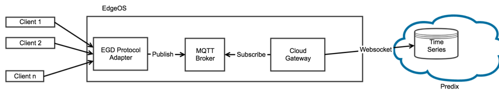
Figure 1. Protocol Adapter - EGD
