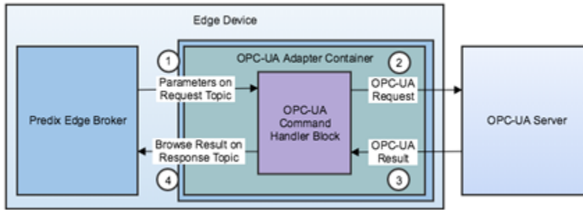
Figure 5. OPC-UA Command Handler Operation Steps
