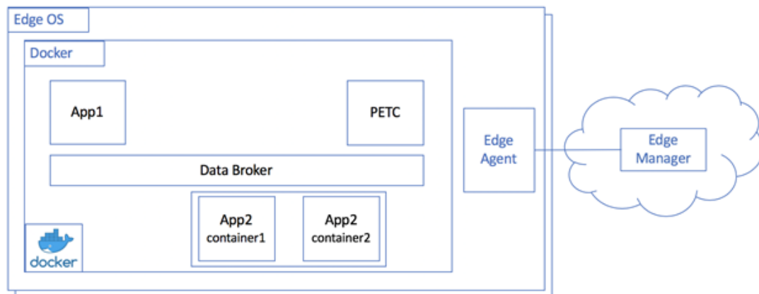
Figure 6. Application Architecture
