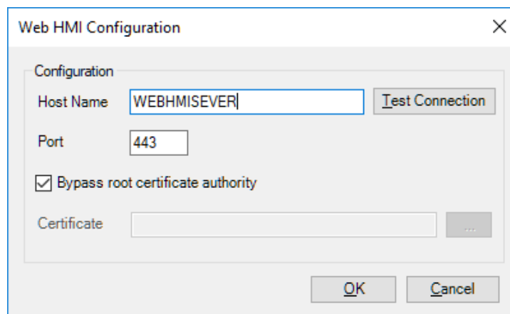
Figure 18 Web HMI Configuration for the OPC UA Server
