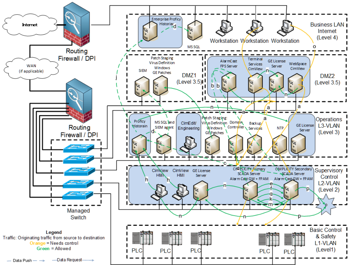
Figure 4 Remote Access to CIMPPLICITY Screens with WebSpace Solution and Terminal Services Solution
