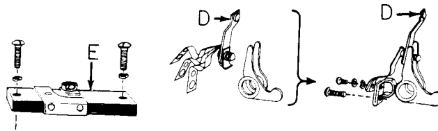
Figure 2: TYPICAL TWO-STAGE SB-1 SWITCH COVER REMOVED
