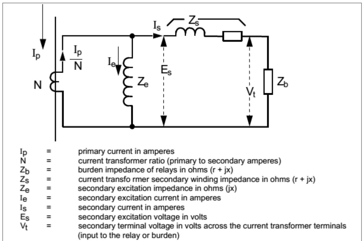
Figure 2: CT equivalent circuit
