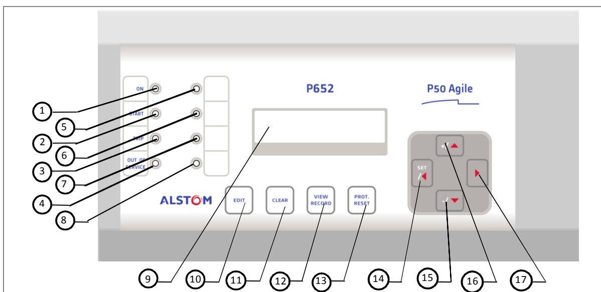
Figure 1: Front panel
