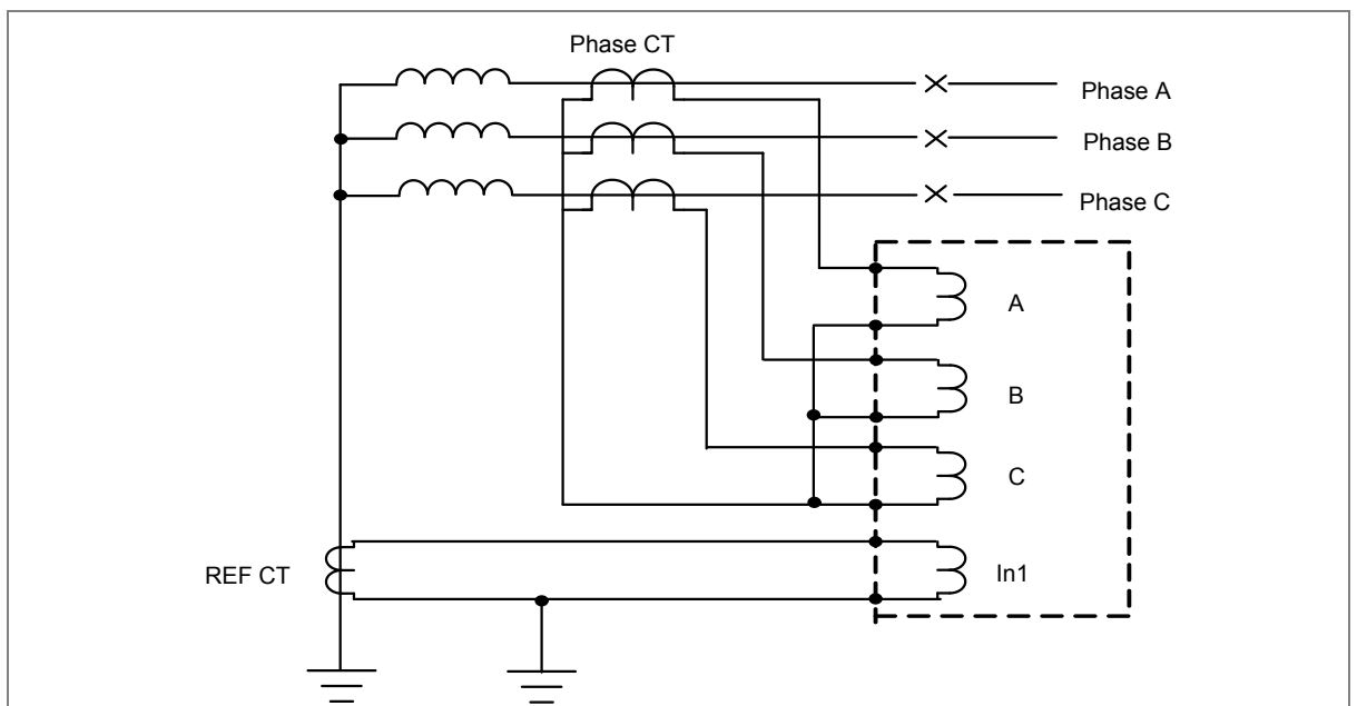
Figure 10: CT connection diagram for low impedance REF application
