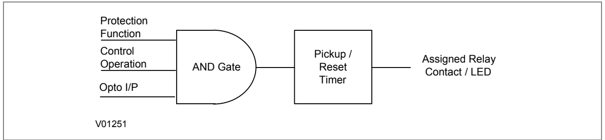
Figure 4: AND logic equation
