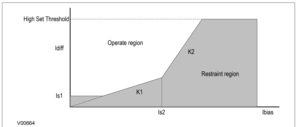
Figure 1: Compensation using biased differential characteristic
