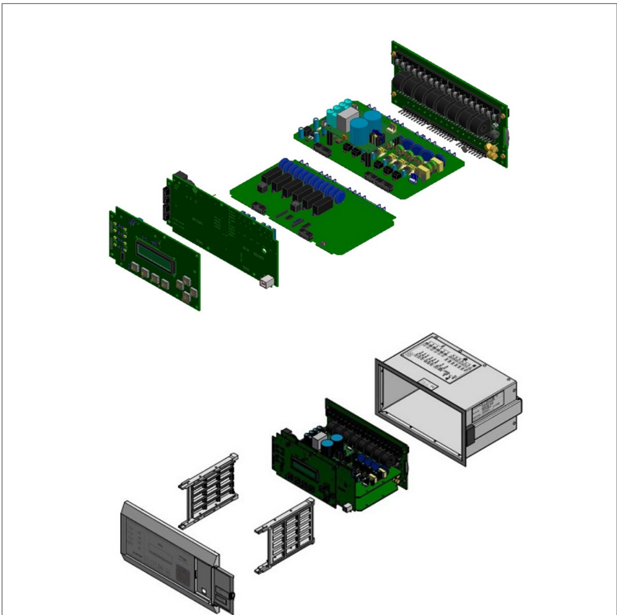
Figure 1: P652 general assembly
