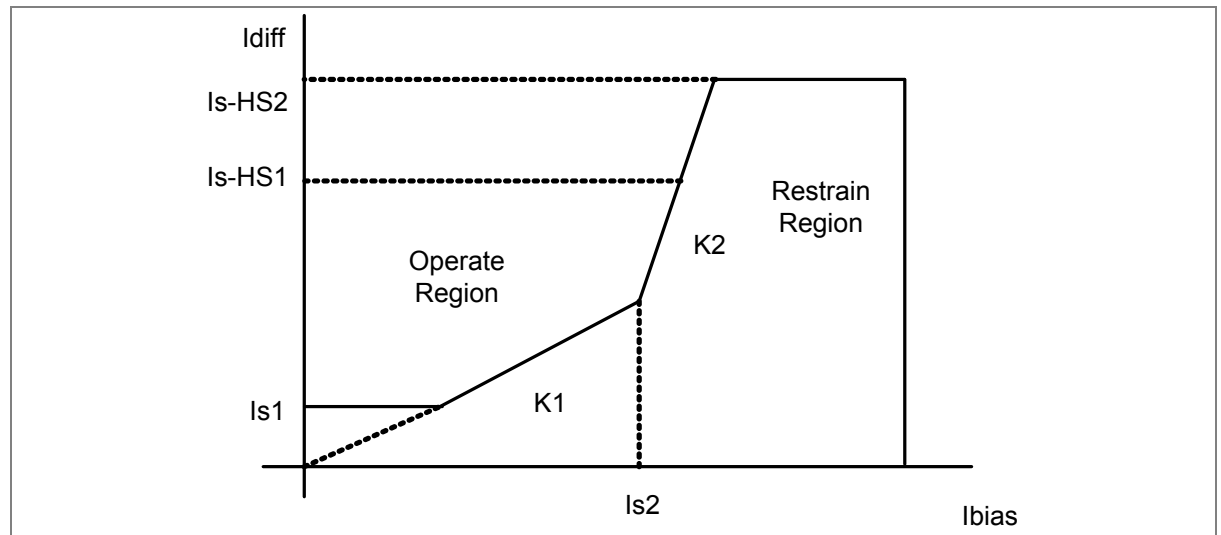
Figure 6: Transformer Differential operating characteristics
