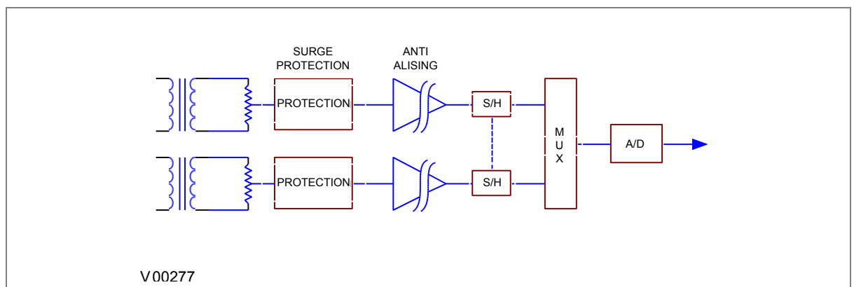
Figure 3: Analog signal processing
