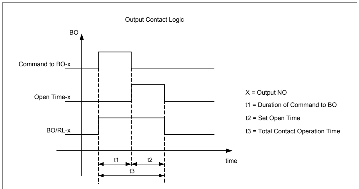
Figure 2: Output contact logic
