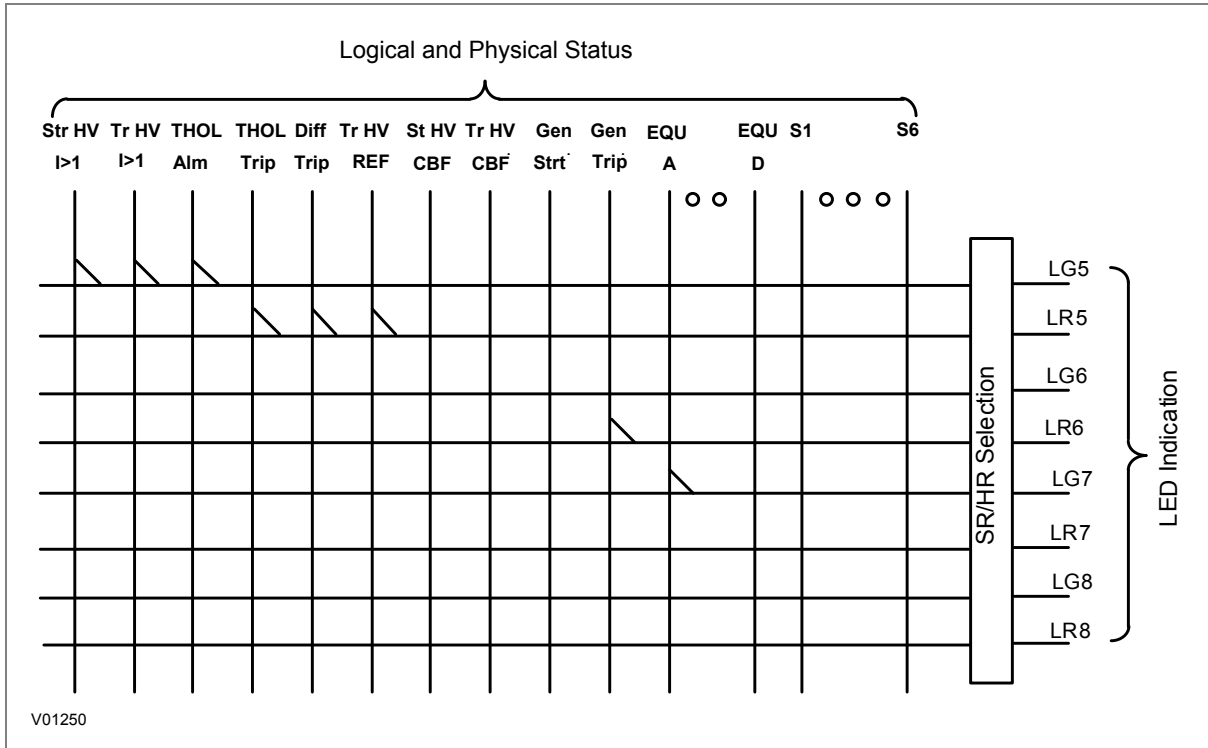
Figure 3: LEDs configuration logic
