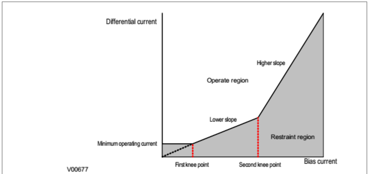
Figure 9: Percentage biased Differential Characteristics for LoZ REF function
