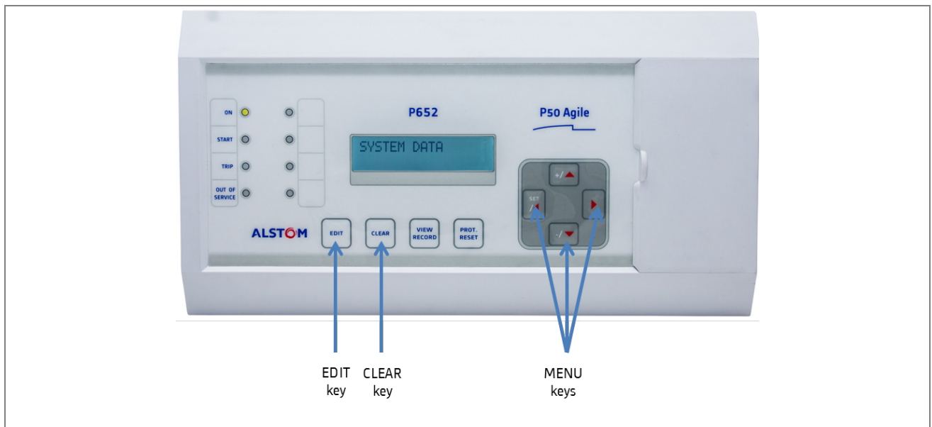
Figure 1: P652 menu/function keys
