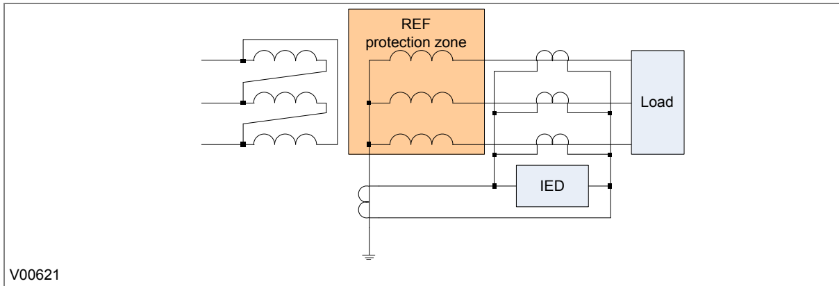
Figure 8: REF protection for star side
