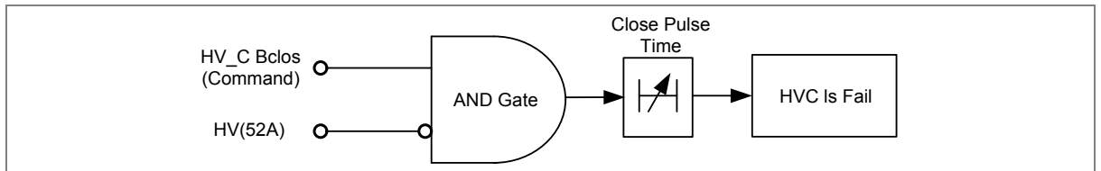
Figure 9: HV CB close fail alarm
