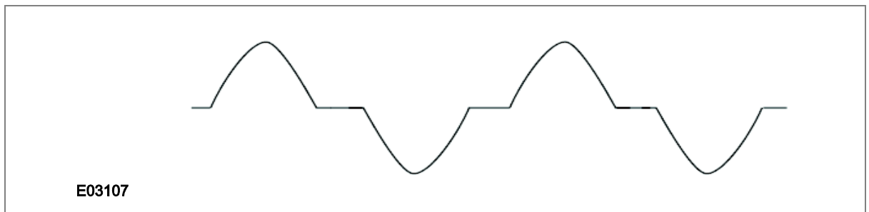
Figure 5: Typical overflux current waveform
