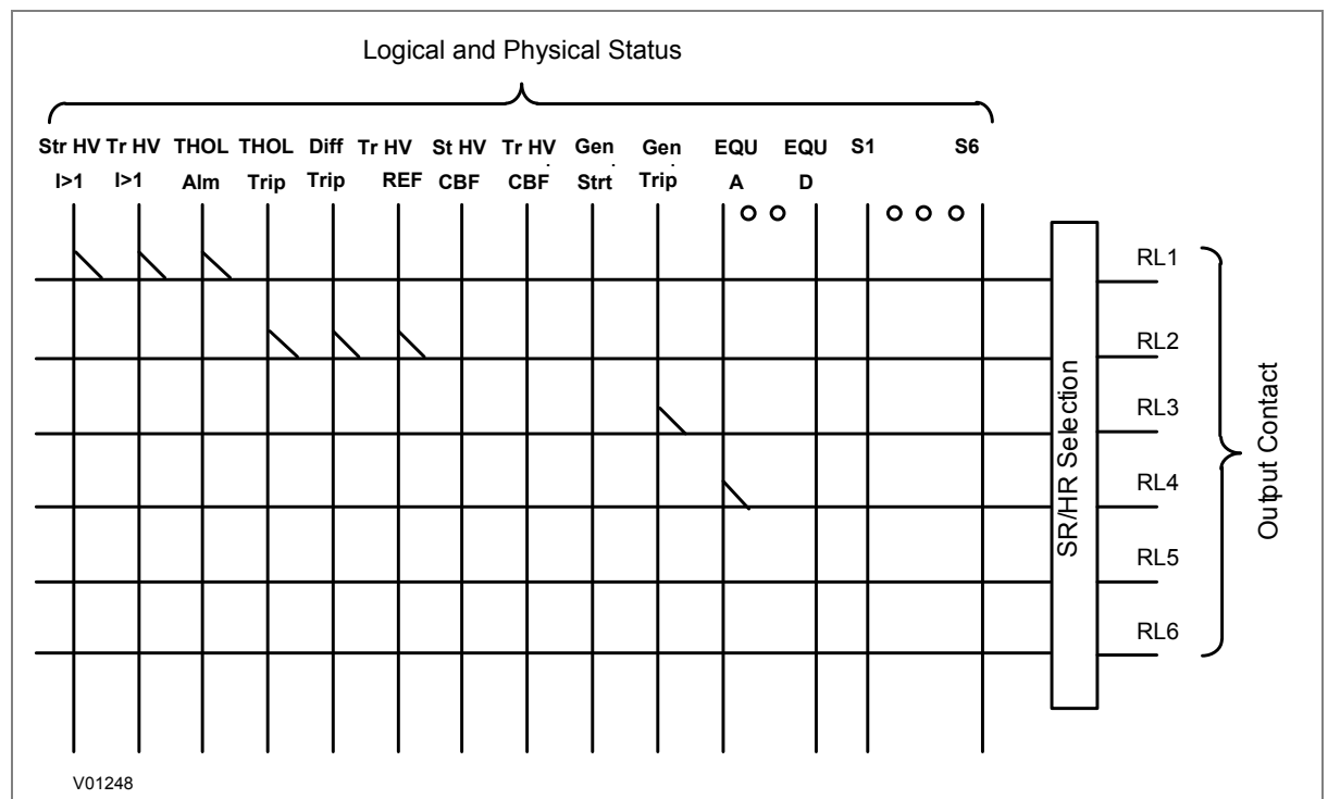
Figure 1: Output contact configuration logic
