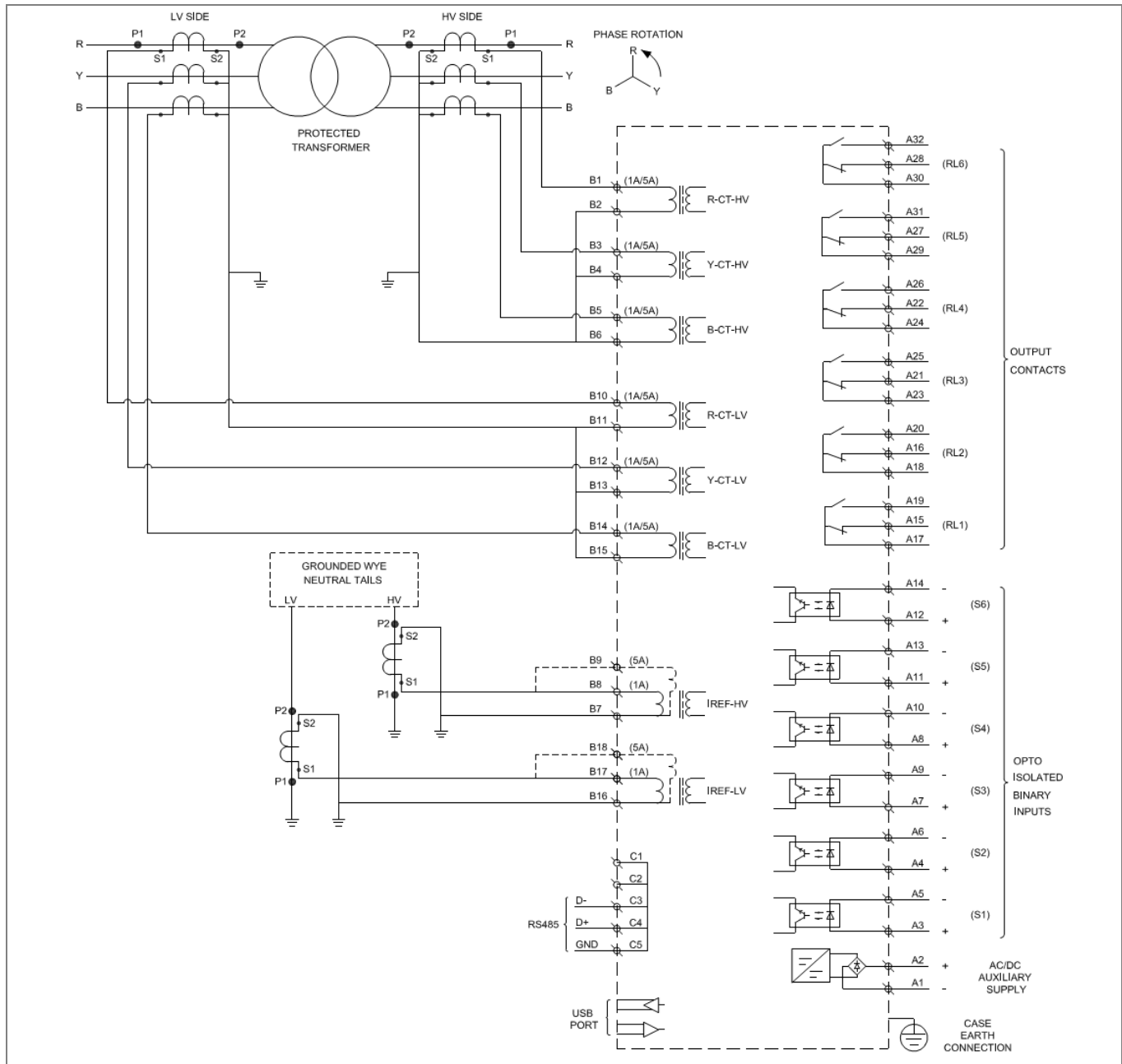
Figure 1: P652 wiring diagram
