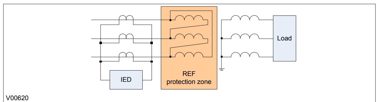
Figure 7: REF protection for delta side
