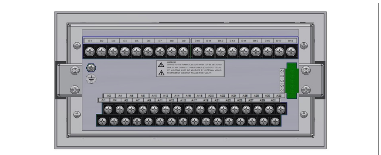
Figure 5: P652 rear view-terminal connection
