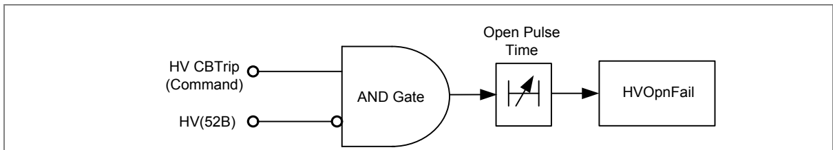
Figure 8: HV CB open fail alarm
