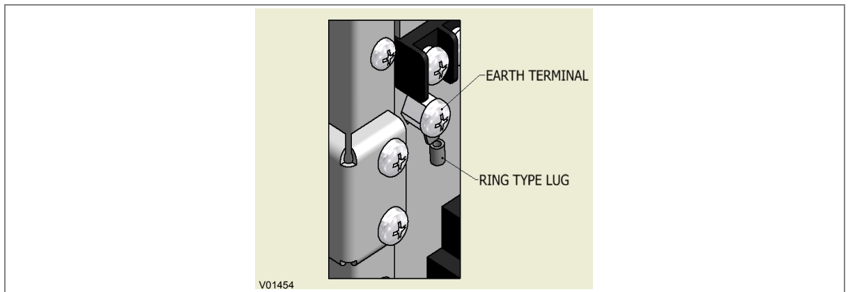
Figure 8: Earthing terminal on the rear side of the relay
