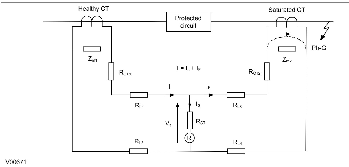
Figure 11: High Impedance principle
