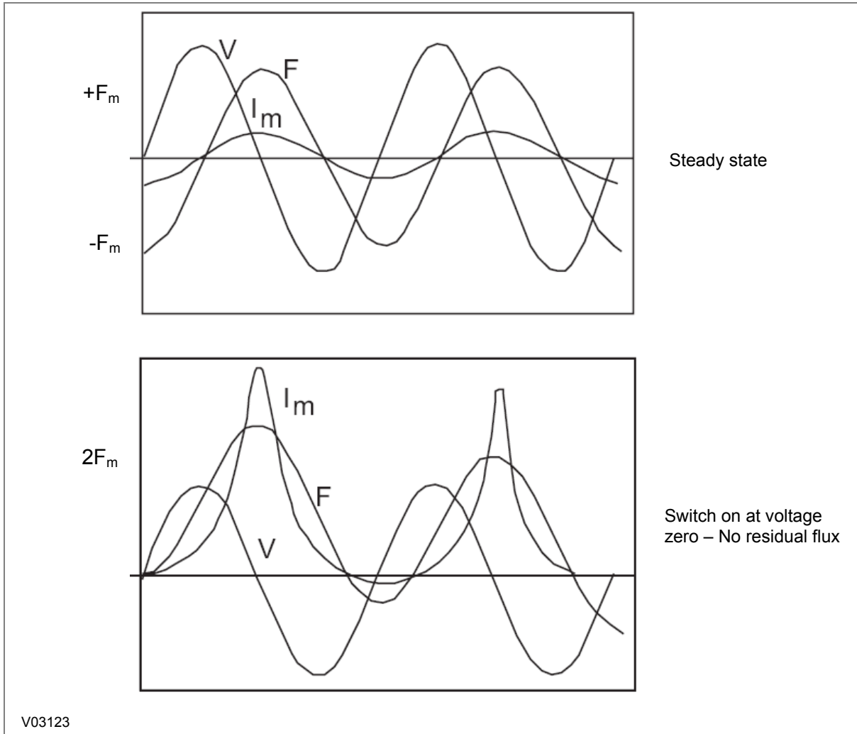
Figure 4: Magnetising inrush phenomenon
