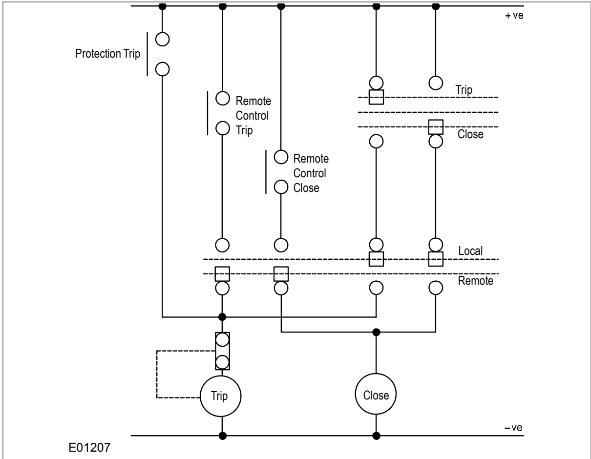
Figure 7: Local and Remote Control of Circuit Breaker
