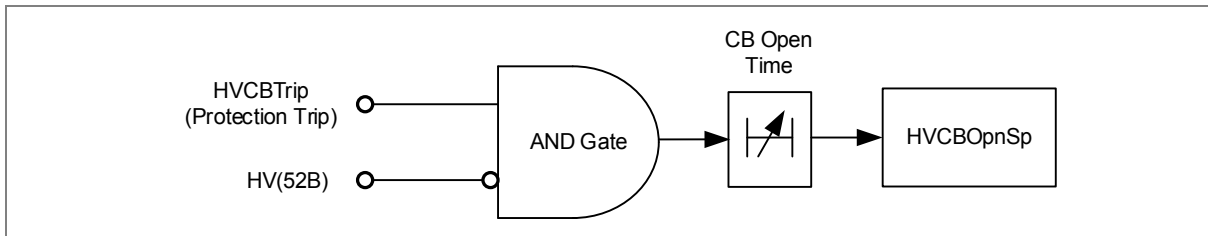
Figure 6: HV CB open supervision logic
