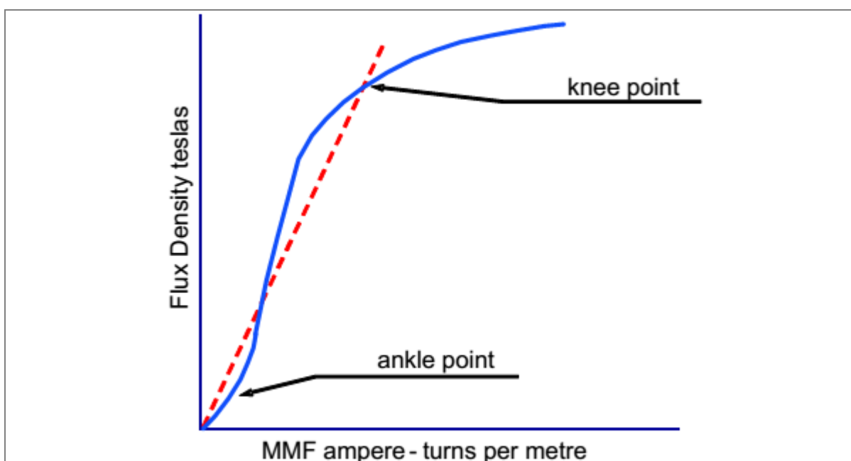
Figure1: Exciting characteristic for a CROSS core CT
