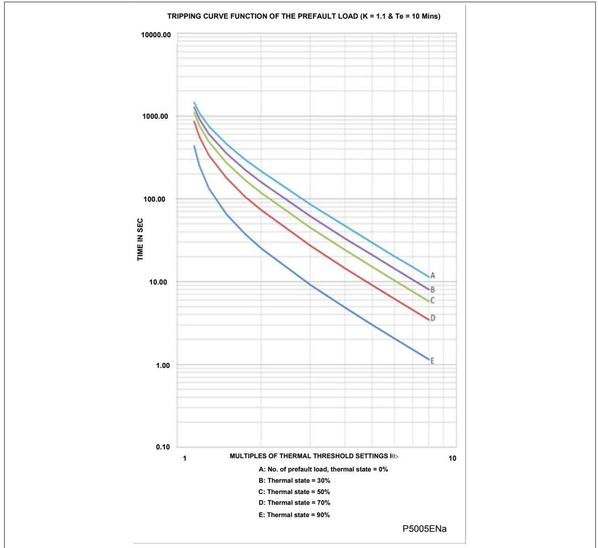
Figure 13: Thermal Overload curve
