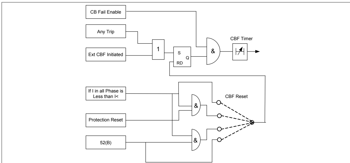
Figure 14: CB Fail logic
