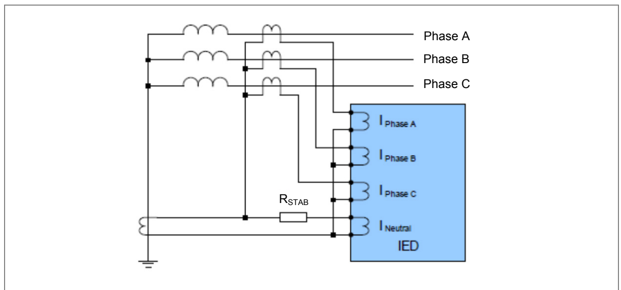
Figure 12: High Impedance REF connection
