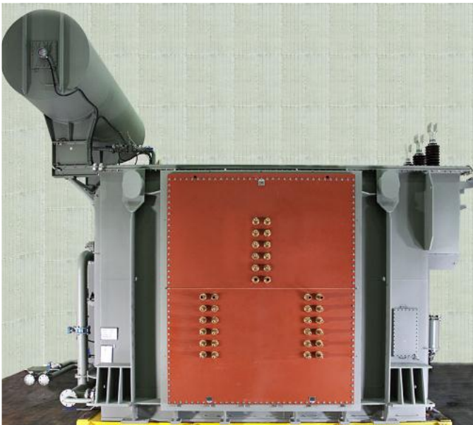
The highest rated 300 MVA EAF power transformer, built for MMK / ATAKAS in 2010
