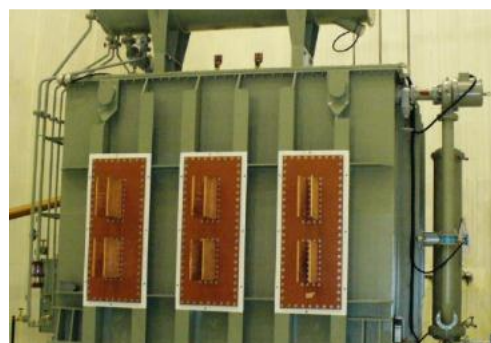
PEAF transformer equipped with flat copper bar bushings
