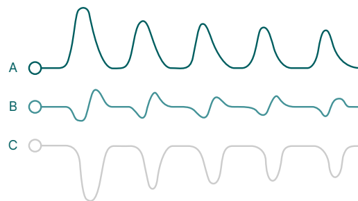
FIGURE 3: Typical magnetizing inrush waveform – showing harmonic distortion
