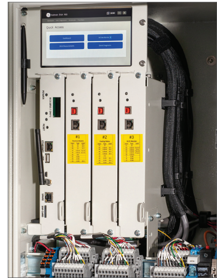
Location of maximum 3 x add-on cards
