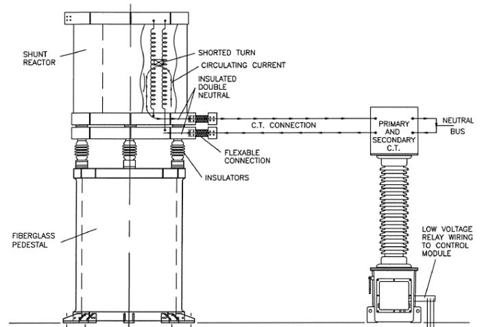
Figure 6C: Split-phase reactor
