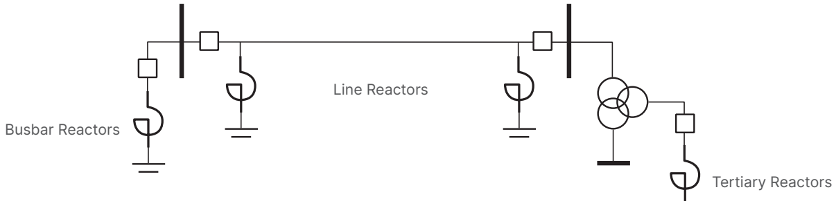
Figure 2: Shunt reactor application in power systems
