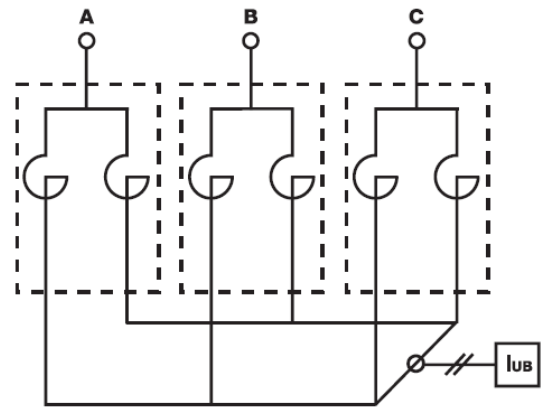
Figure 6A: Differential protection with split-phase shunt reactors.
