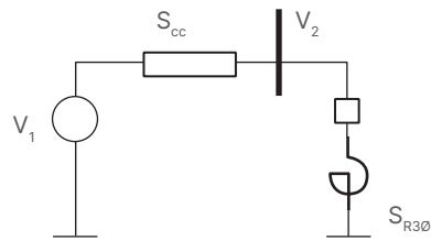
Figure 4: Practical circuit for voltage control analysis
