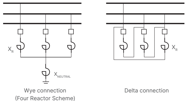
Figure 3: Winding connection of shunt reactors.
