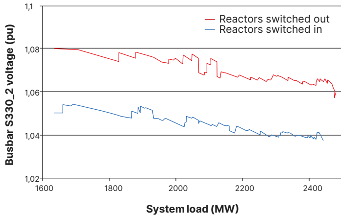
Figure 5: Voltage response with shunt reactors switched in/out.
