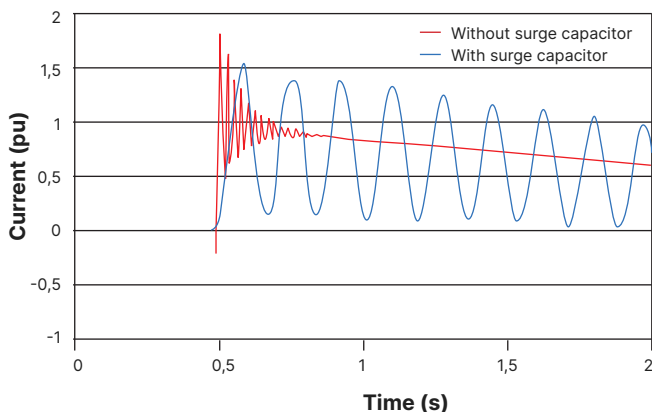
Figure 7: Switching transient frequency with/without surge capacitors.
