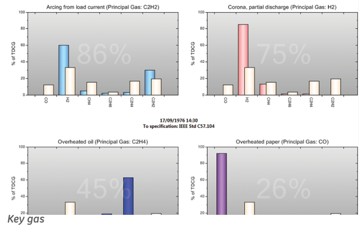
Figure 2: DGA models help provide clear indication of changes that may signal an evolving incipient fault condition in transformers.
