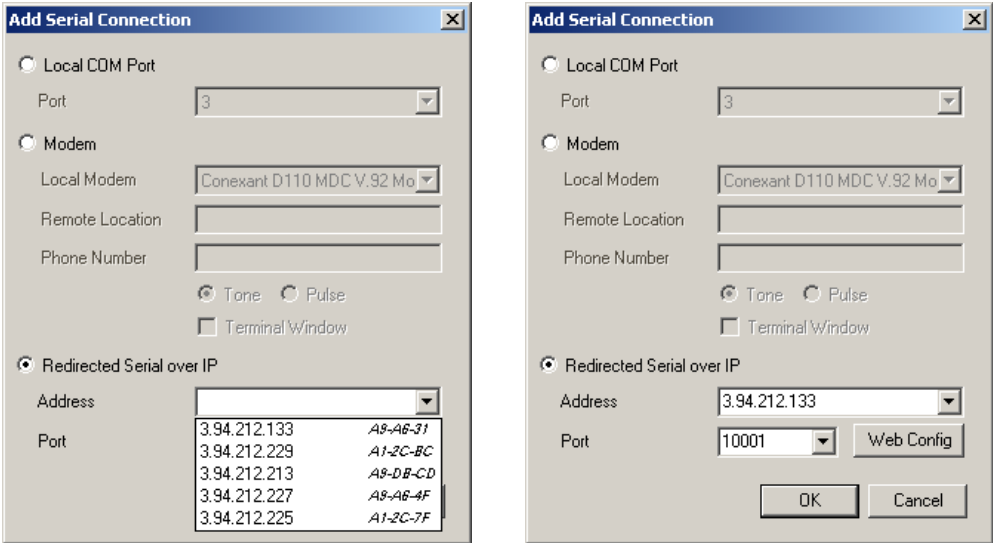
Figure 20: Add Serial Connection View: Selecting Xport device and TCP port
