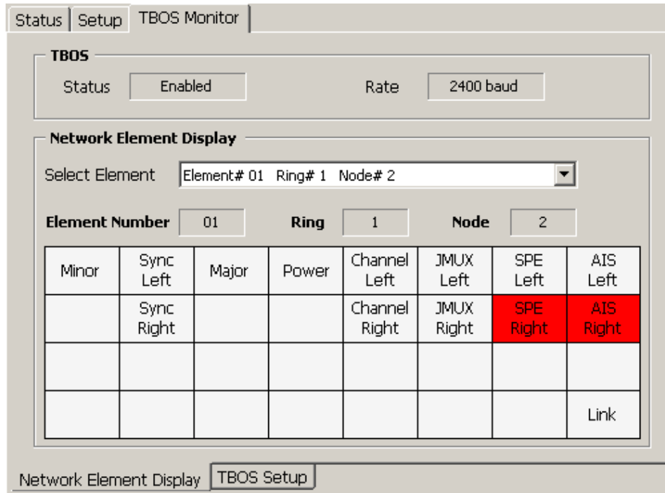
Figure 17: TBOS Monitor Tab – Network Element Display Sub-Tab
