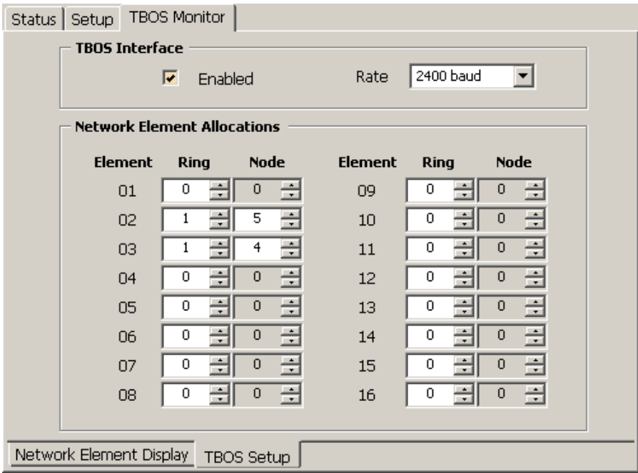
Figure 18: TBOS Monitor Tab – TBOS Setup Sub-Tab
