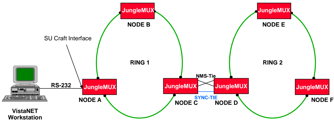
Figure 1: Visibility of two JungleMUX rings on one VistaNET workstation
