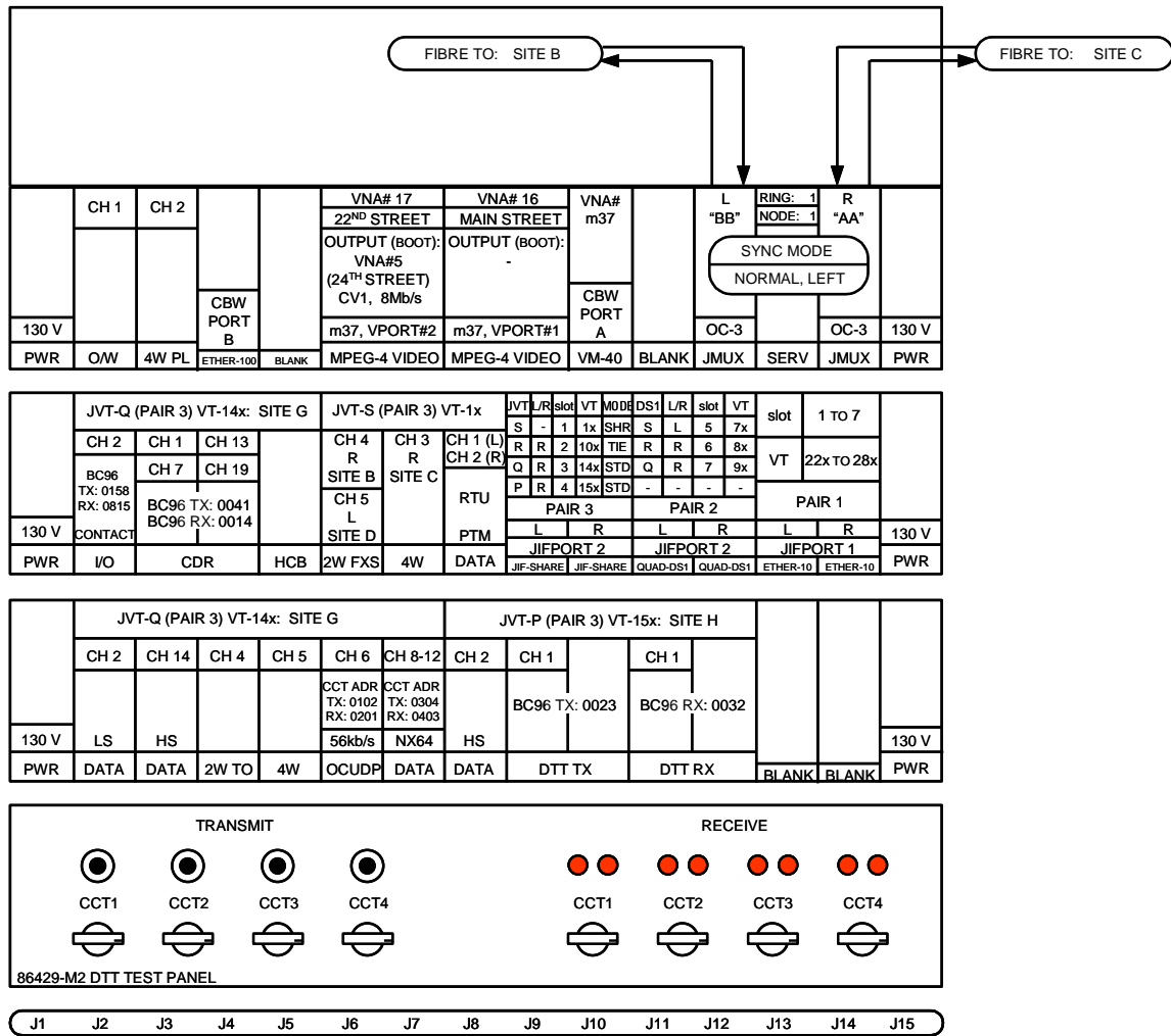
Figure 9: Typical Rack Layout for a JungleMUX SONET Node
