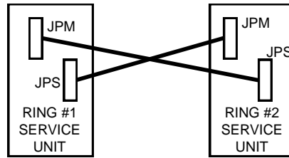
TWO RING JPACK CONNECTION
