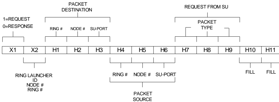
Figure 8: 13-Byte Header Details
