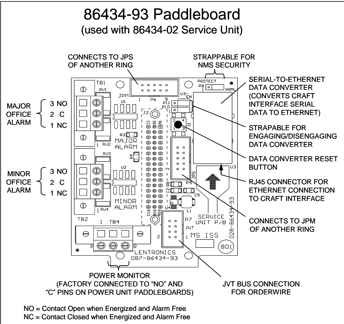
Figure 12: 86434-93 Service Unit Paddleboard Connections
