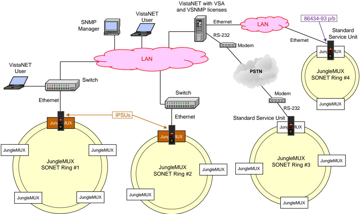
Figure 3: Control of two separate JungleMUX systems with IPSUs installed
