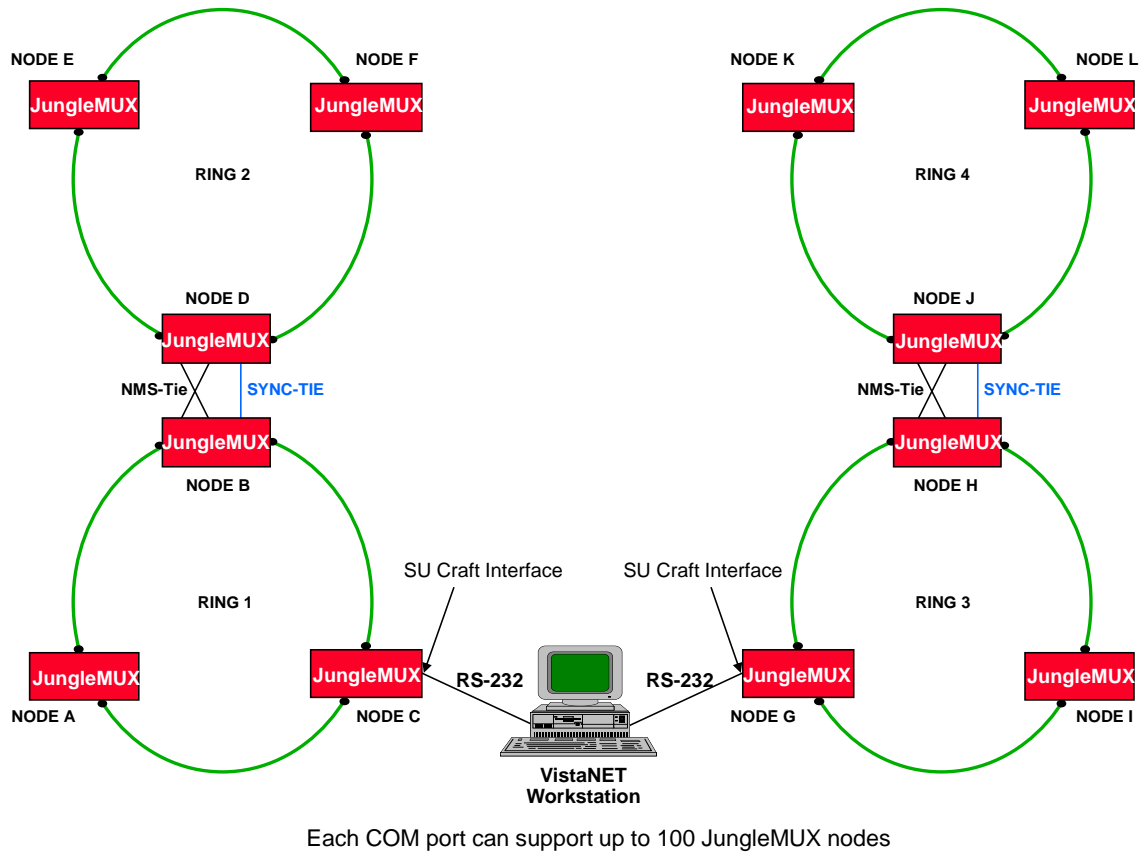
Figure 2: Visibility of two separate JungleMUX systems on one VistaNET PC
