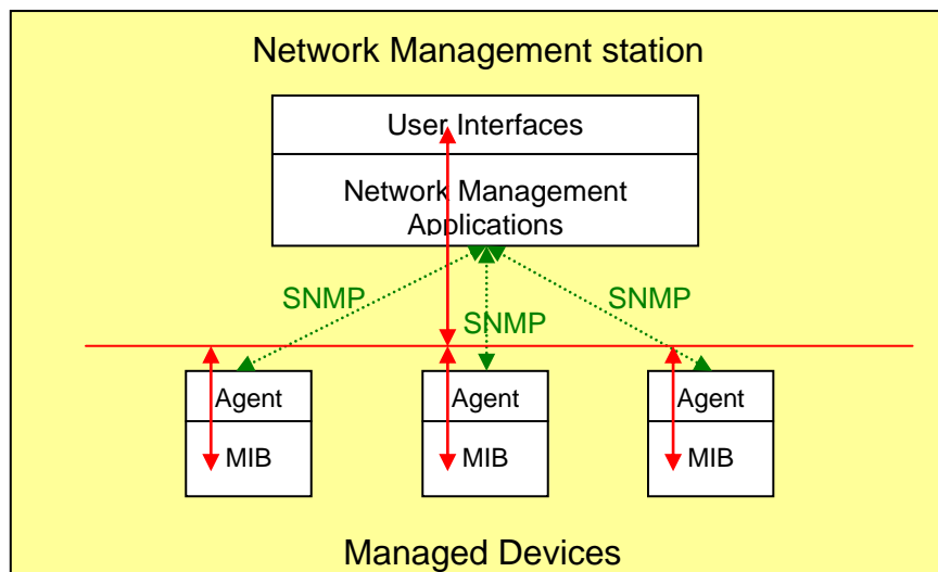
Figure 23: SNMP Model
