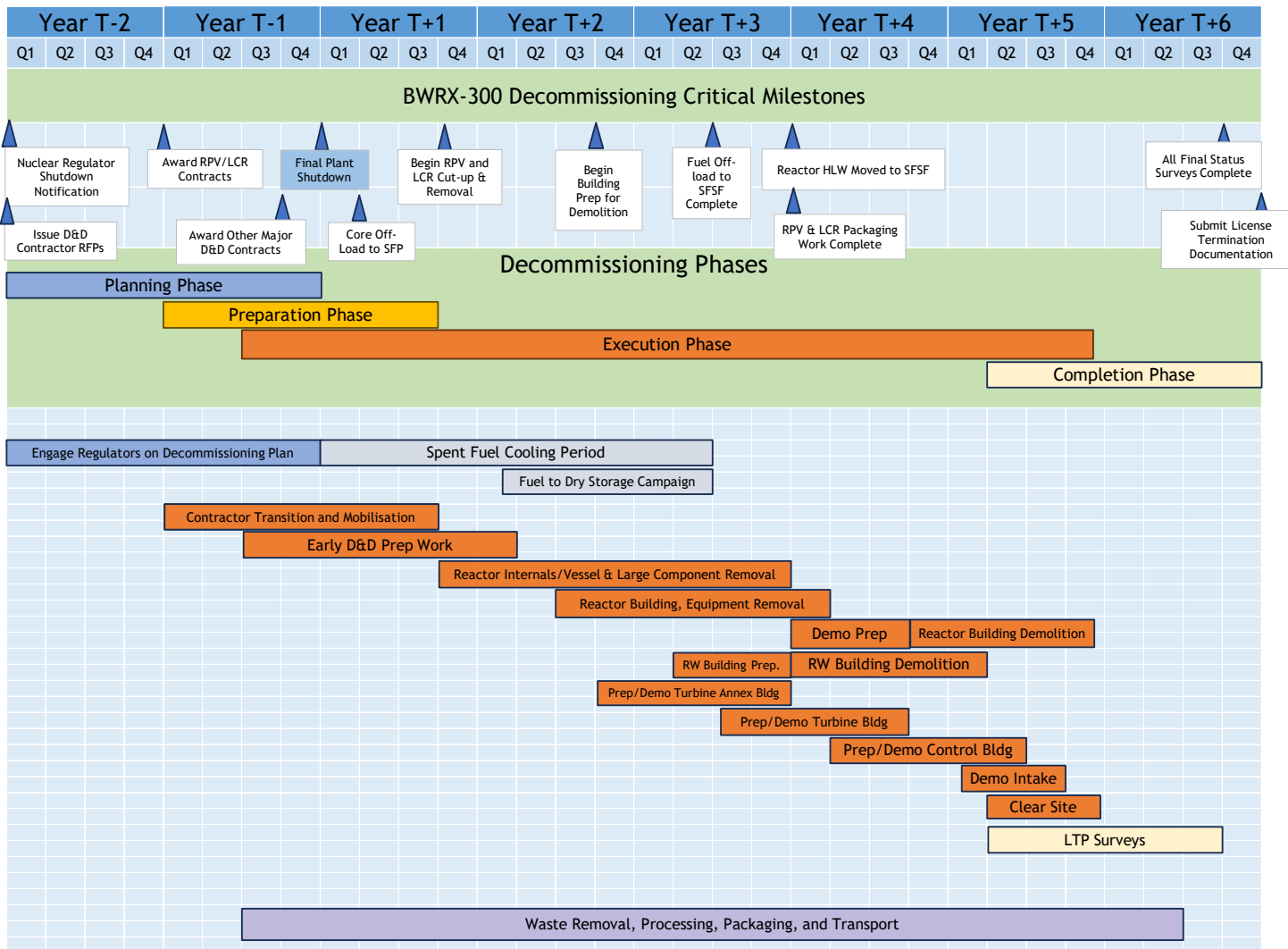
Figure 21-1: BWRX-300 Decommissioning Critical Milestones
